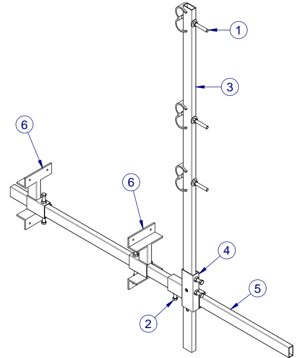
ISOMETRIC VIEW
